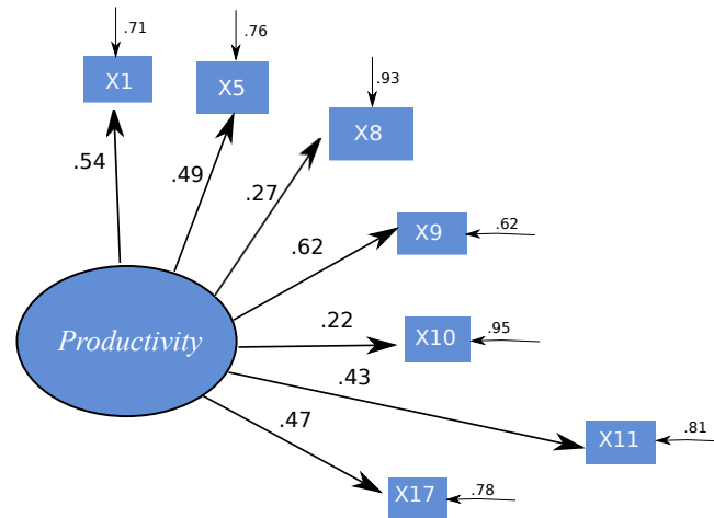
Figure 7.3: Model II with Loadings with Company Selected Seven Factors of Productivity of Software Development
