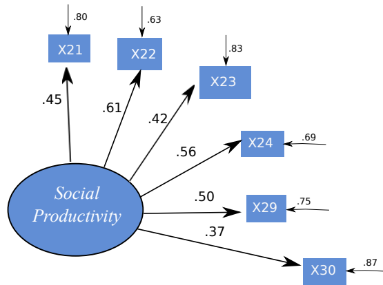
Figure 7.4: Model III with Loadings for Six Factors of Social Productivity for Software Development
