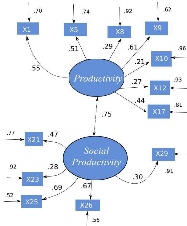
Figure 7.8: Model VII for Productivity and Social Productivity in a Software Development Organization
