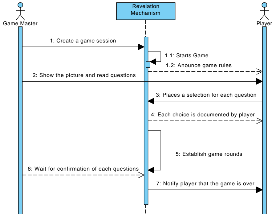
Figure 4.1: The Sequential Steps of the Game of Revealing Personality Traits
