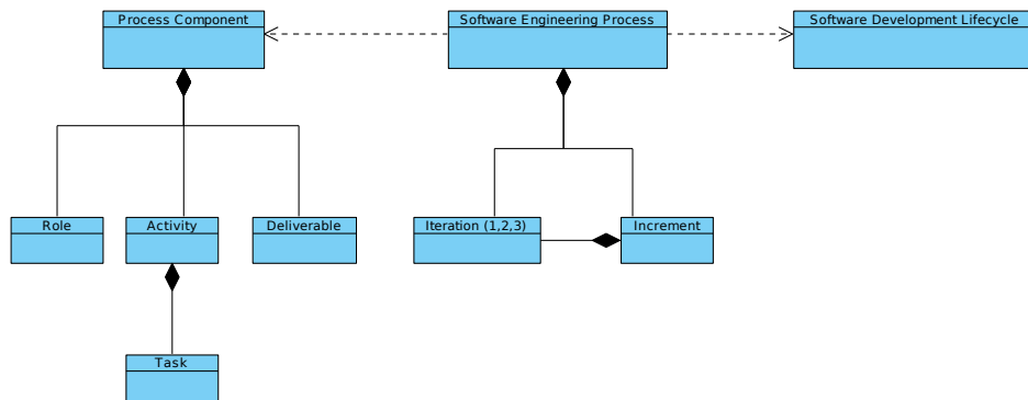
Figure 2.1: A Meta-Model for Software Engineering Process.
